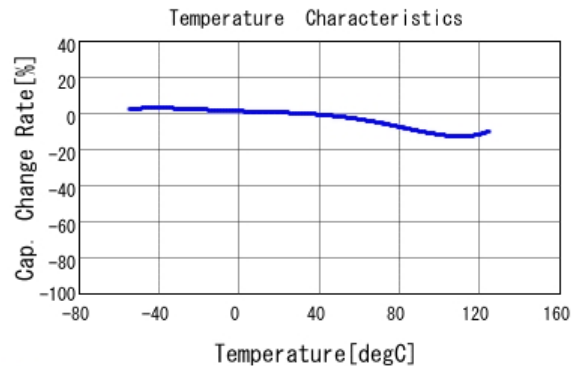
■ GR442QR73D102KW01 C-Temp. capchange, DCOV, AC1Vrms
