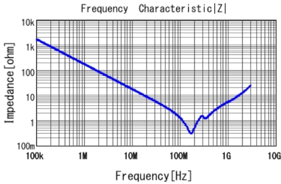
■ GR442QR73D102KW01 |Z| DCOV, 25degC
