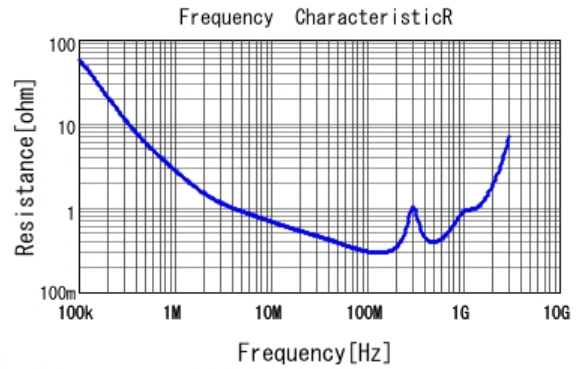
■ GR442QR73D102KW01 R DCOV, 25degC
