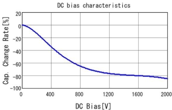
■ GR442QR73D102KW01 C-DC bias capchange, 25.0degC, AC1V
