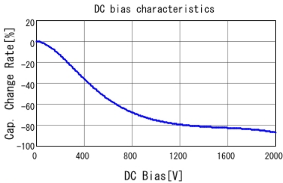
■ GR443DR73D472KW01 C-DC bias capchange, 25.0degC, AC1V
