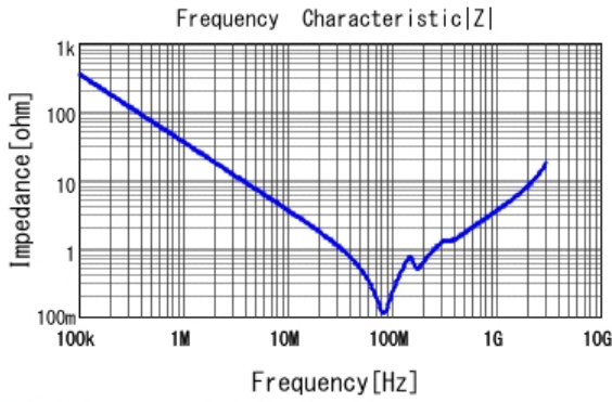
■ GR443DR73D472KW01 |Z| DCOV, 25degC
