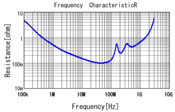
■ GR443DR73D472KW01 R DCOV, 25degC
