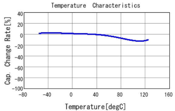
■ GR443DR73D472KW01 C-Temp. capchange, DCOV, AC1Vrms
