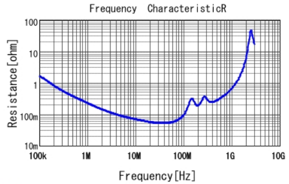
■ GR455DR73D103KW01 R DC0V, 25degC
