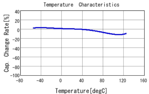
■ GR455DR73D103KW01 C-Temp. capchange, DC0V, AC1Vrms
