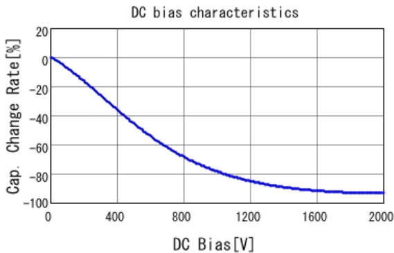
■ GR455DR73D103KW01 C-DC bias capchange, 25.0degC, AC1V
