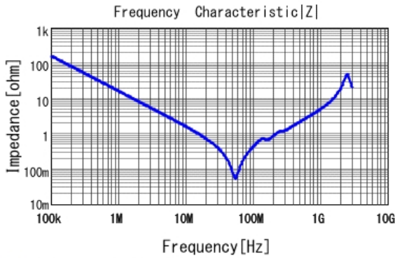
■ GR455DR73D103KW01 |Z| DC0V, 25degC
