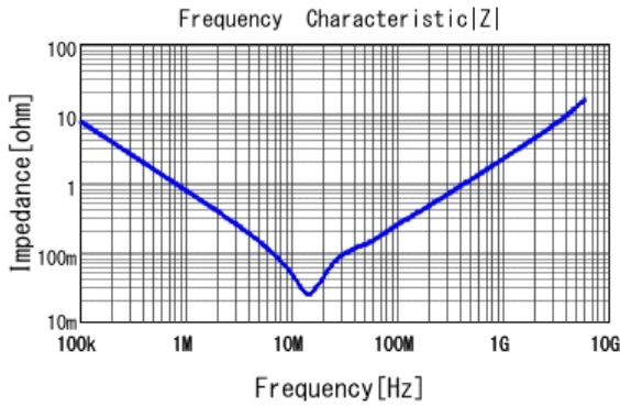
■ GRJ188R71E224KE11 |Z| DCOV, 25degC
