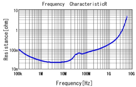
■ GRJ188R71E224KE11 R DCOV, 25degC
