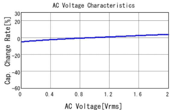
■ GRJ188R71E224KE11 C-AC Voltage capchange, DCOV, 25.0d
