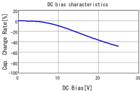
■ GRJ188R71E224KE11 C-DC bias capchange, 25.0degC, AC1.
