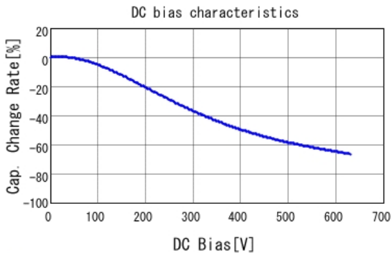
■ GRJ31BR72J222KWJ1 C-DC bias capchange, 25.0degC, AC1V
