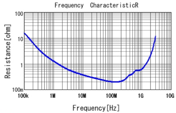
■ GRJ31BR72J222KWJ1 R DCOV, 25degC
