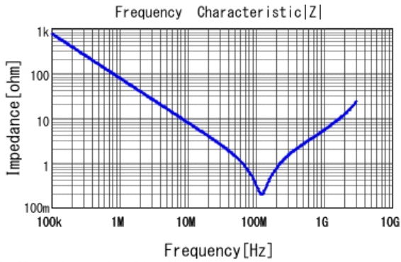
■ GRJ31BR72J222KWJ1 |Z| DCOV, 25degC
