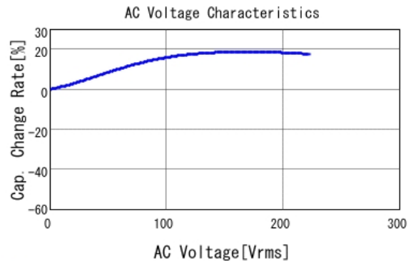
■ GRJ31BR72J222KWJ1 C-AC Voltage capchange, DCOV, 25.0d
