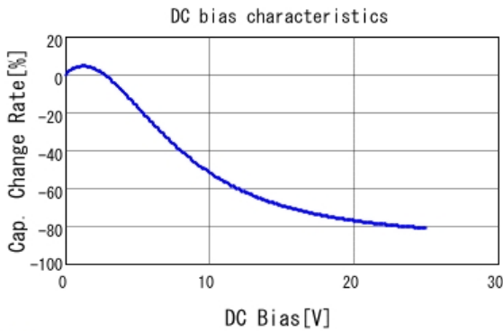
■ GRJ31CR61E106KE11 C-DC bias capchange, 25.0degC, AC1.
