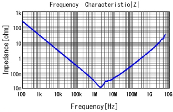
■ GRJ31CR61E106KE11 |Z| DC0V, 25degC
