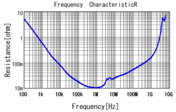
■ GRJ31CR61E106KE11 R DC0V, 25degC
