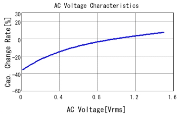
■ GRJ31CR61E106KE11 C-AC Voltage capchange, DC0V, 25.0d
