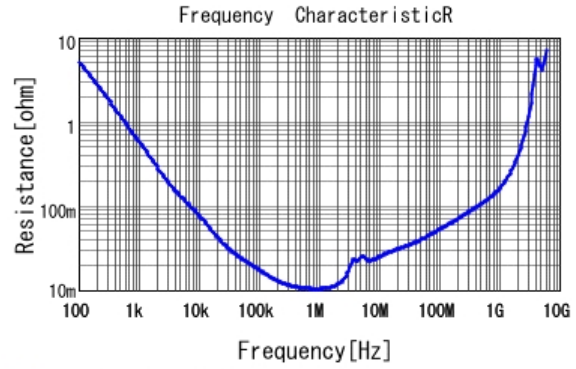
■ GRJ31CR71C106KE11 R DCOV, 25degC
