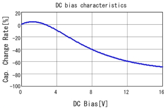
■ GRJ31CR71C106KE11 C-DC bias capchange, 25.0degC, AC1.
