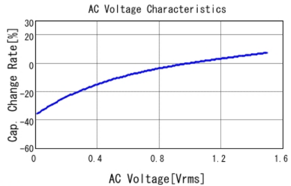
■ GRJ31CR71C106KE11 C-AC Voltage capchange, DCOV, 25.0d
