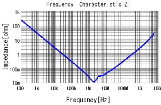
■ GRJ31CR71C106KE11 |Z| DCOV, 25degC
