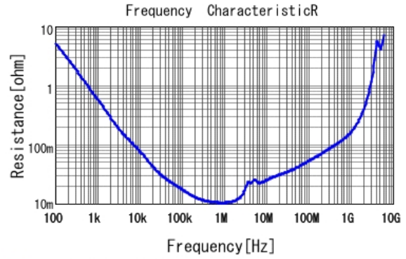
■ GRJ31CR71E106KE11 R DC0V, 25degC
