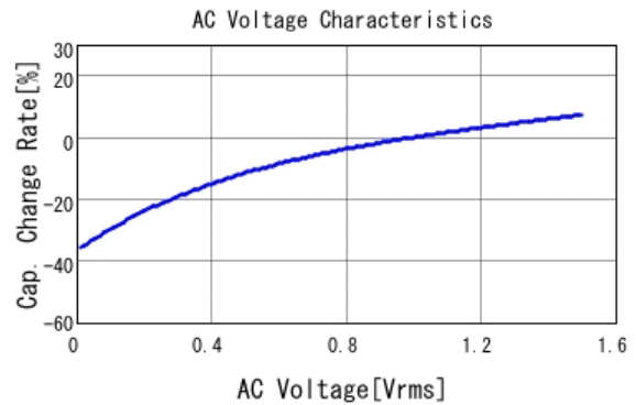
■ GRJ31CR71E106KE11 C-AC Voltage capchange, DC0V, 25.0d
