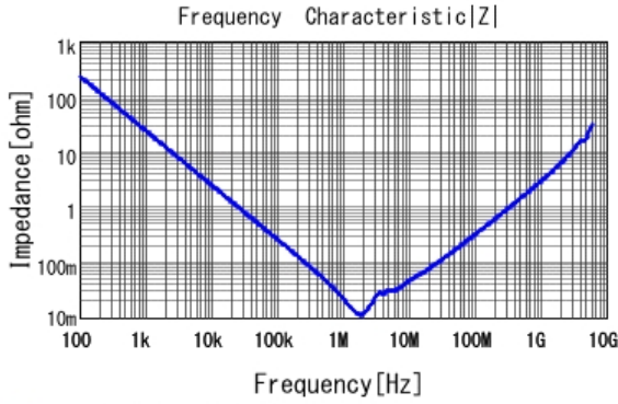
■ GRJ31CR71E106KE11 |Z| DC0V, 25degC
