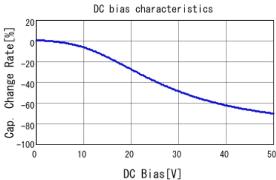
■ GRJ31CR71H225KE11 C-DC bias capchange, 25.0degC, AC1.
