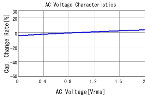
■ GRJ31CR71H225KE11 C-AC Voltage capchange, DCOV, 25.0d
