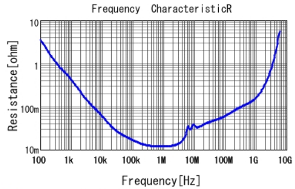
■ GRJ31CR71H225KE11 R DCOV, 25degC
