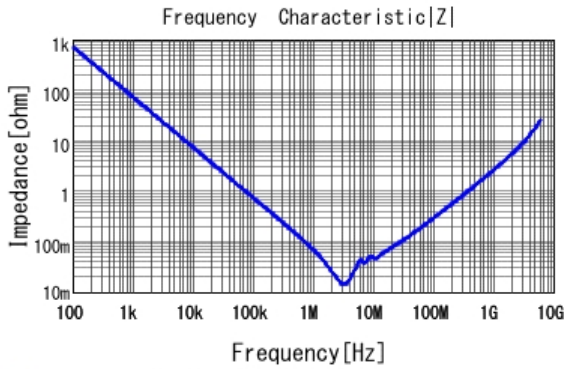
■ GRJ31CR71H225KE11 |Z| DCOV, 25degC
