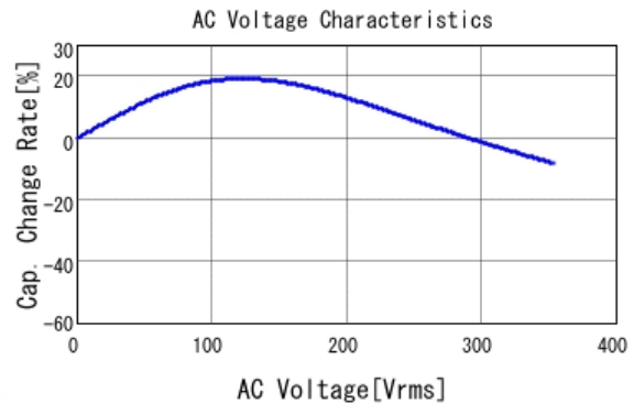
■ GRJ31CR73A103KWJ3 C-AC Voltage capchange, DCOV, 25.0d
