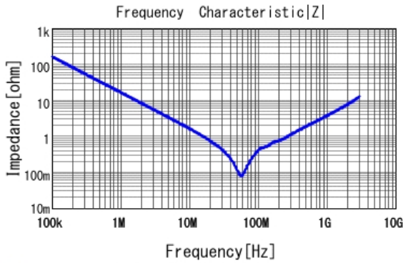
■ GRJ31CR73A103KWJ3 |Z| DCOV, 25degC
