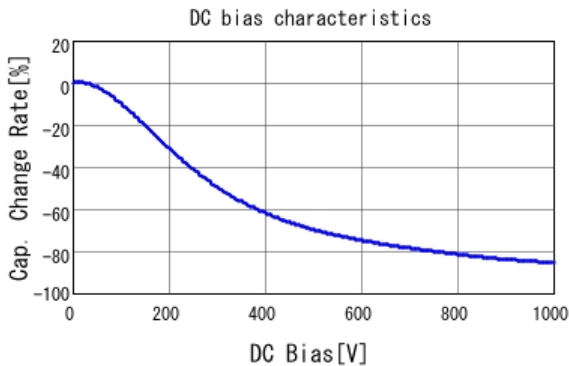
■ GRJ31CR73A103KWJ3 C-DC bias capchange, 25.0degC, AC1V
