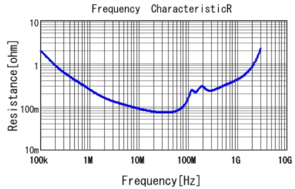
■ GRJ31CR73A103KWJ3 R DCOV, 25degC
