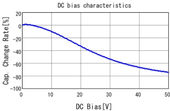
■ GRJ32EC71H106KE11 C-DC bias capchange, 25.0degC, AC1.
