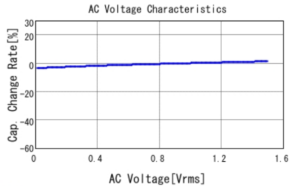
■ GRJ32EC71H106KE11 C-AC Voltage capchange, DC0V, 25.0d
