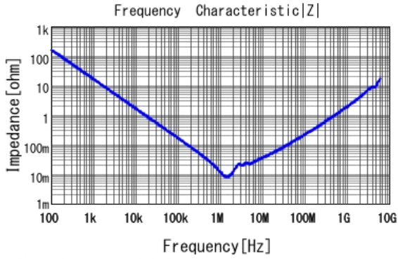
■ GRJ32EC71H106KE11 |Z| DC0V, 25degC
