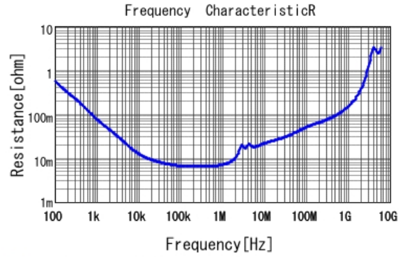
■ GRJ32EC71H106KE11 R DC0V, 25degC
