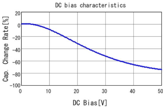
■ GRJ32ER71H106KE11 C-DC bias capchange, 25.0degC, AC1V
