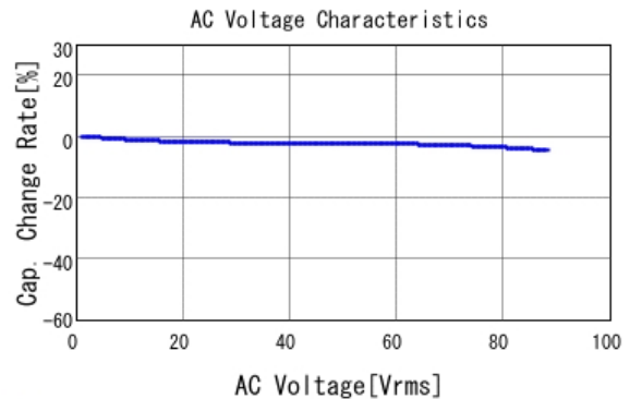
■ GRJ55DR72E105KWJ1 C-AC Voltage capchange, DC0V, 25.0d
