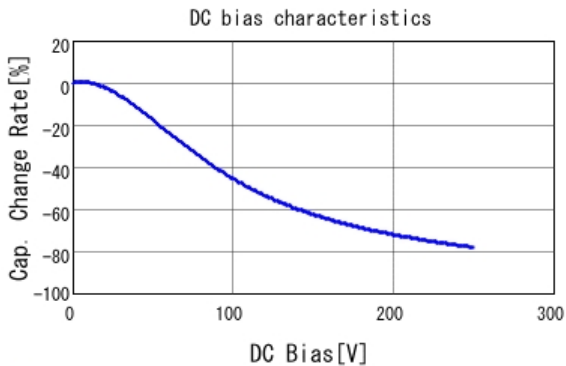
■ GRJ55DR72E105KWJ1 C-DC bias capchange, 25.0degC, AC1V
