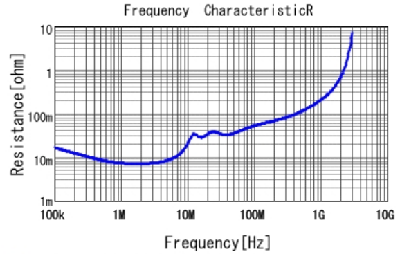
■ GRJ55DR72E105KWJ1 R DC0V, 25degC
