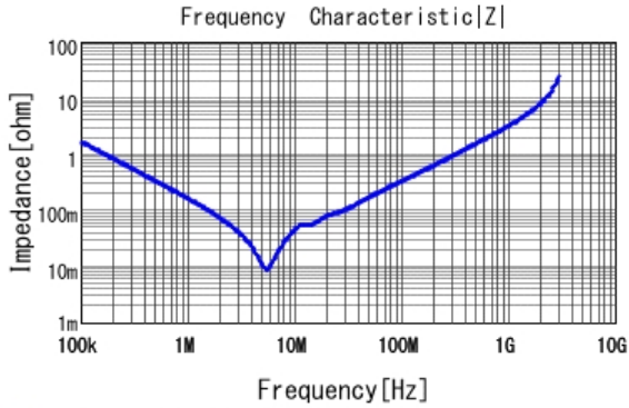
■ GRJ55DR72E105KWJ1 |Z| DC0V, 25degC
