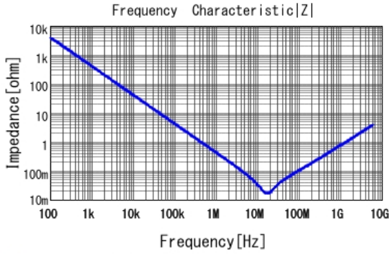
■ GRM022R60J474ME15 |Z| DCOV, 25degC
