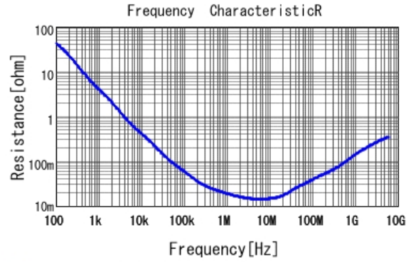
■ GRM022R60J474ME15 R DCOV, 25degC
