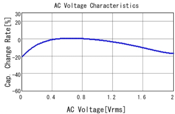
■ GRM022R60J474ME15 C-AC Voltage capchange, DCOV, 25.0d
