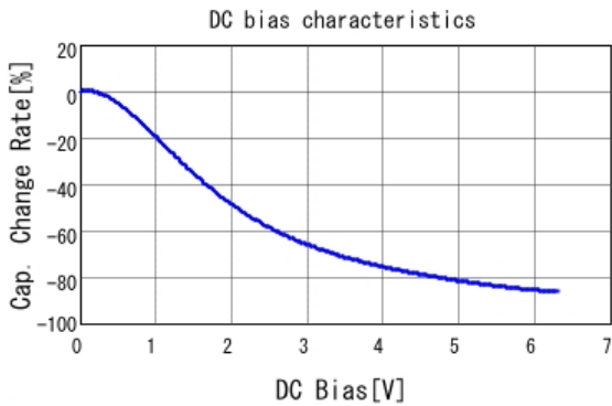
■ GRM022R60J474ME15 C-DC bias capchange, 25.0degC, AC0.
