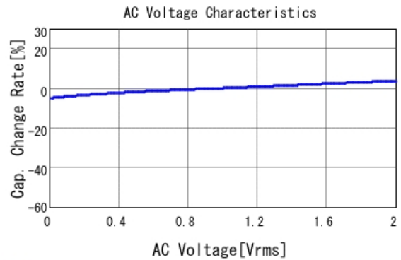
■ GRM022R71A331KA01 C-AC Voltage capchange, DCOV, 25.0d
