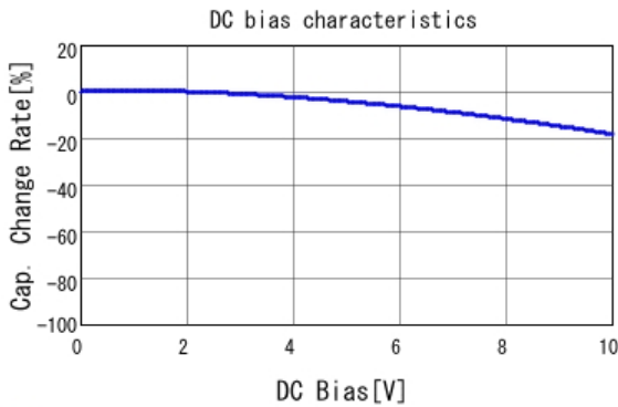
■ GRM022R71A331KA01 C-DC bias capchange, 25.0degC, AC1.
