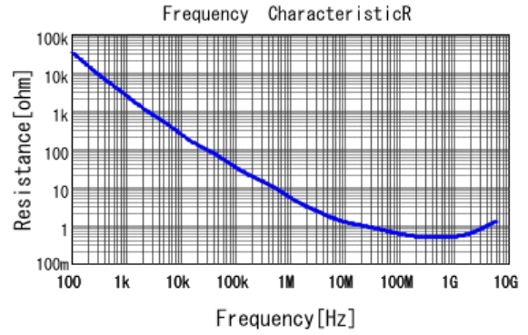
■ GRM022R71A331KA01 R DCOV, 25degC
