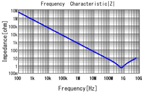
■ GRM022R71A331KA01 |Z| DCOV, 25degC
