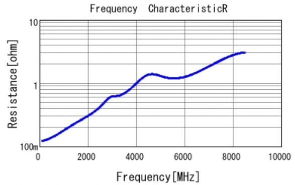
■ GRM0332C1H680GA01 R DCOV, 20degC
