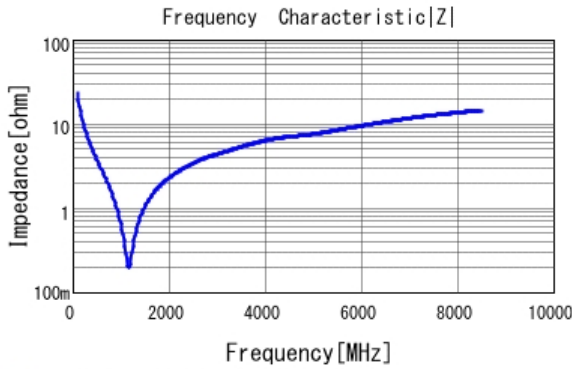
■ GRM0332C1H680GA01 |Z| DCOV, 20degC
