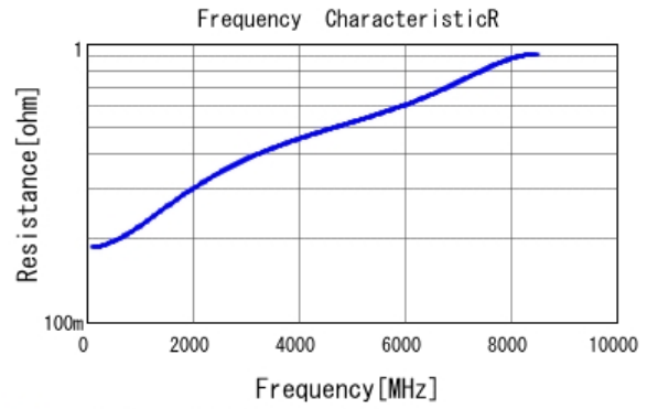
■ GRM0332C1H8R0WA01 R DCOV, 20degC
