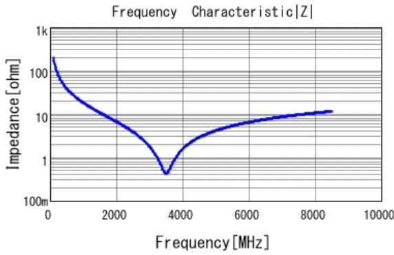
■ GRM0332C1H8R0WA01 |Z| DCOV, 20degC
