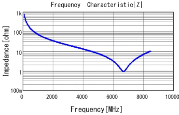
■ GRM0333C1H2R2WA01 |Z| DCOV, 20degC
