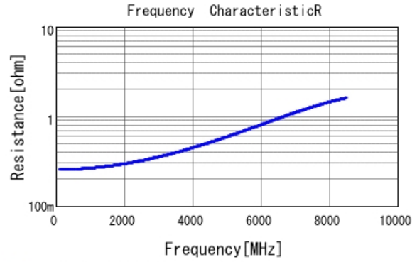
■ GRM0333C1H2R7WA01 R DCOV, 20degC
