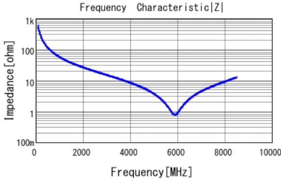
■ GRM0333C1H2R7WA01 |Z| DCOV, 20degC
