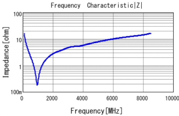
■ GRM0335C1E101FA01 |Z| DCOV, 25degC
