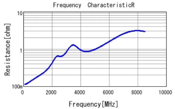
■ GRM0335C1E101FA01 R DCOV, 25degC
