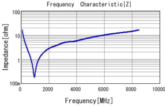
■ GRM0335C1E101JA01 |Z| DCOV, 25degC
