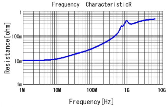
■ GRM0335C1E102JA01 R DCOV, 25degC
