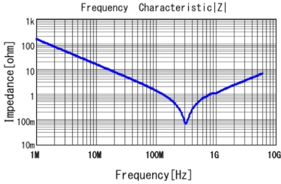
■ GRM0335C1E102JA01 |Z| DCOV, 25degC
