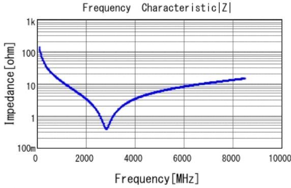
■ GRM0335C1E120JA01 |Z| DCOV, 25degC
