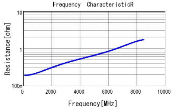
■ GRM0335C1E120JA01 R DCOV, 25degC
