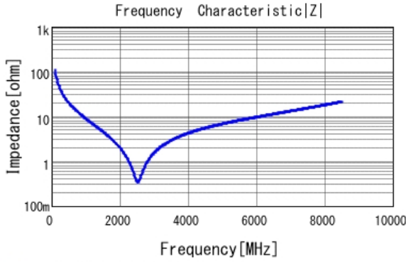
■ GRM0335C1E150JA01 |Z| DCOV, 25degC
