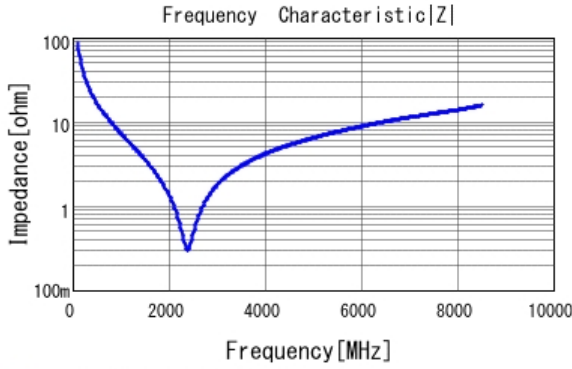
■ GRM0335C1E180JA01 |Z| DCOV, 25degC
