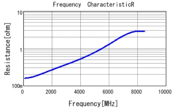
■ GRM0335C1E180JA01 R DCOV, 25degC
