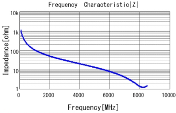
■ GRM0335C1E1R5BA01 |Z| DC0V, 25degC
