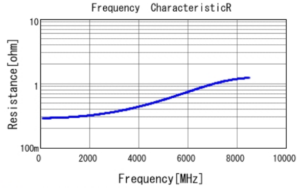
■ GRM0335C1E1R5BA01 R DC0V, 25degC
