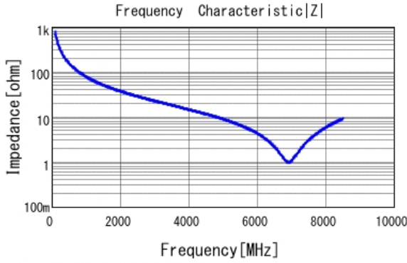
■ GRM0335C1E2R0BA01 |Z| DCOV, 25degC
