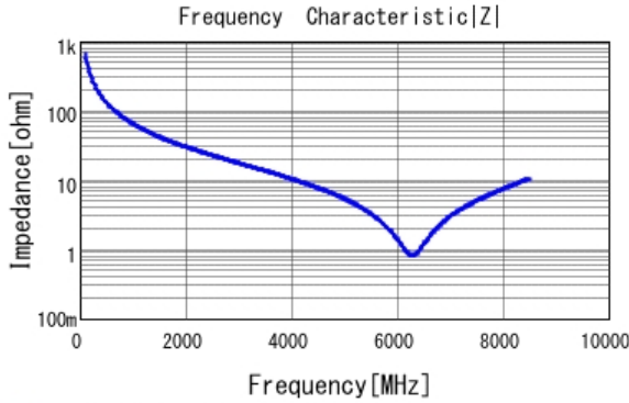
■ GRM0335C1E2R4CA01 |Z| DCOV, 25degC
