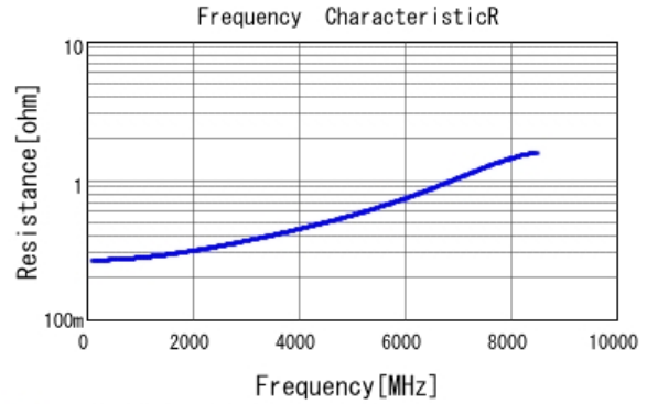
■ GRM0335C1E2R4CA01 R DCOV, 25degC
