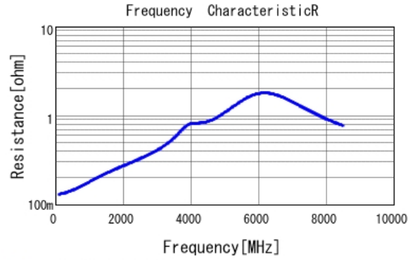
■ GRM0335C1E390JA01 R DCOV, 25degC
