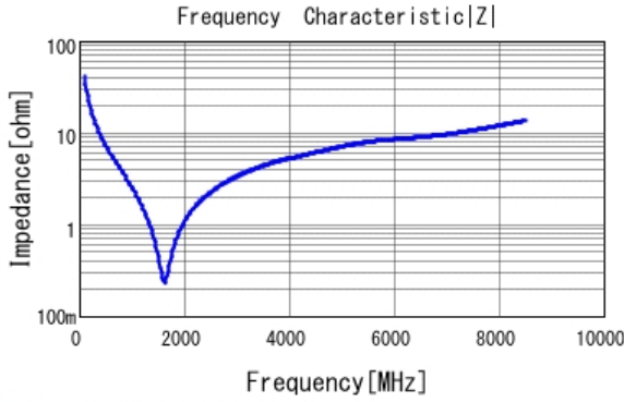
■ GRM0335C1E390JA01 |Z| DCOV, 25degC
