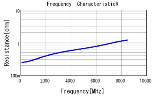
■ GRM0335C1E3R0BA01 R DCOV, 25degC
