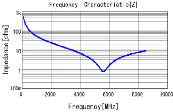
■ GRM0335C1E3R0BA01 |Z| DCOV, 25degC
