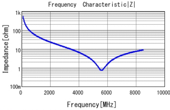
■ GRM0335C1E3R0CA01 |Z| DCOV, 25degC
