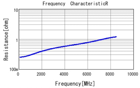
■ GRM0335C1E3R0CA01 R DCOV, 25degC
