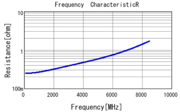
■ GRM0335C1E3R3CA01 R DCOV, 25degC
