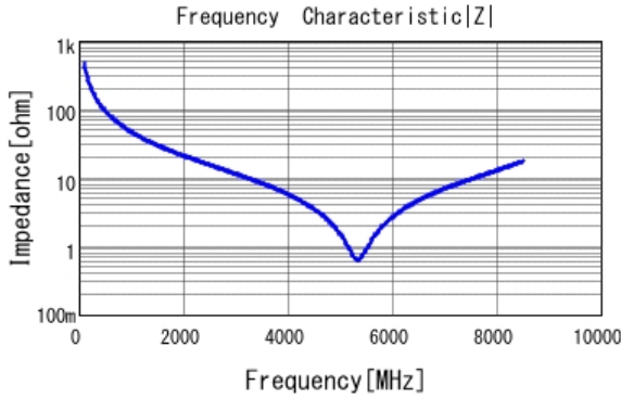
■ GRM0335C1E3R3CA01 |Z| DCOV, 25degC
