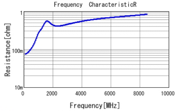
■ GRM0335C1E471GA01 R DCOV, 25degC
