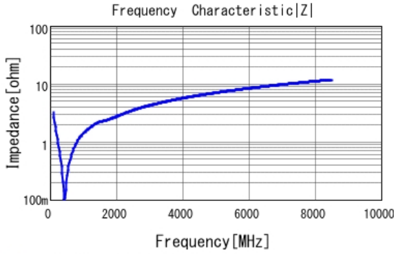
■ GRM0335C1E471GA01 |Z| DCOV, 25degC
