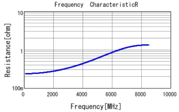
■ GRM0335C1E4R0CA01 R DCOV, 25degC
