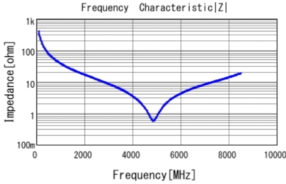
■ GRM0335C1E4R0CA01 |Z| DCOV, 25degC
