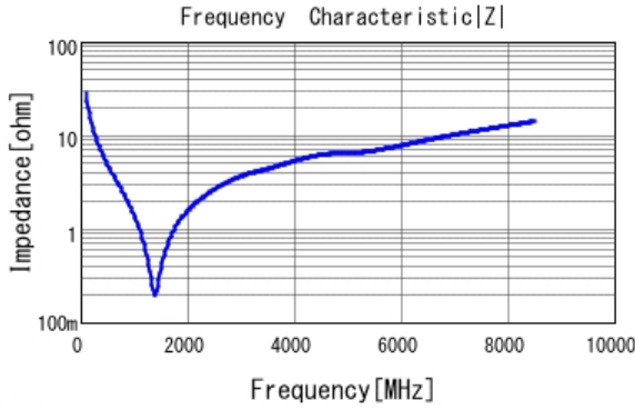
■ GRM0335C1E560JA01 |Z| DCOV, 25degC
