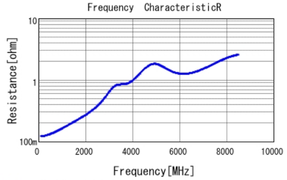
■ GRM0335C1E560JA01 R DCOV, 25degC
