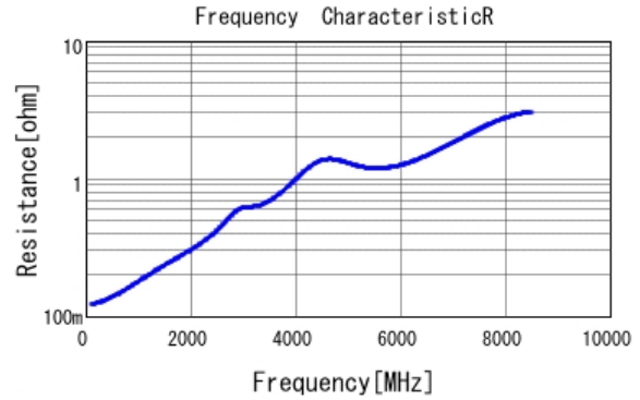
■ GRM0335C1E680JA01 R DCOV, 25degC
