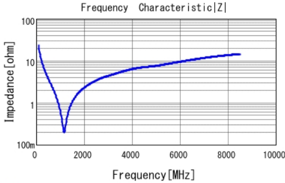
■ GRM0335C1E680JA01 |Z| DCOV, 25degC
