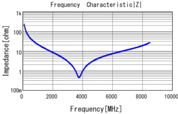
■ GRM0335C1E6R8CA01 |Z| DCOV, 25degC
