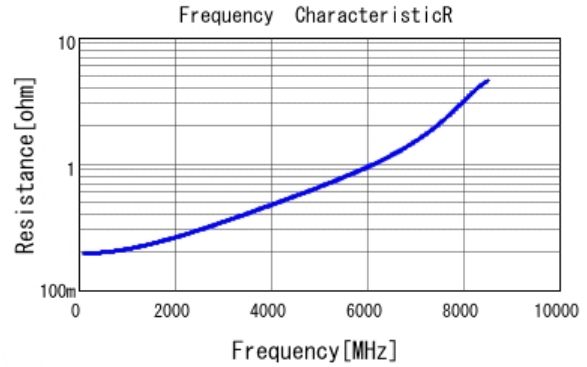
■ GRM0335C1E6R8CA01 R DCOV, 25degC
