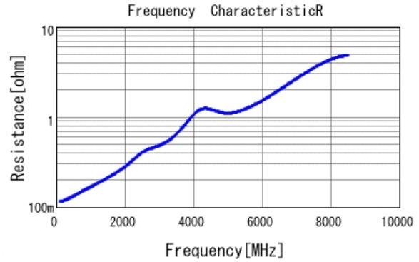
■ GRM0335C1E820JA01 R DCOV, 25degC
