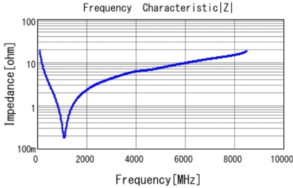
■ GRM0335C1E820JA01 |Z| DCOV, 25degC
