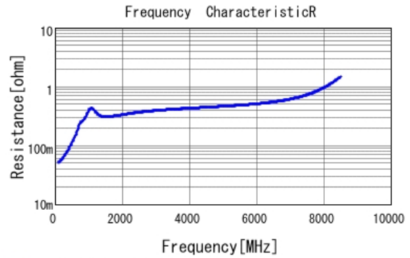
■ GRM0335C1E821JA01 R DCOV, 25degC
