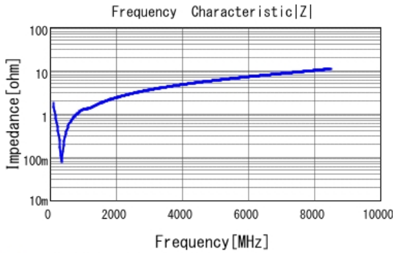
■ GRM0335C1E821JA01 |Z| DCOV, 25degC
