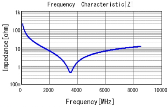
■ GRM0335C1E8R0CA01 |Z| DCOV, 25degC
