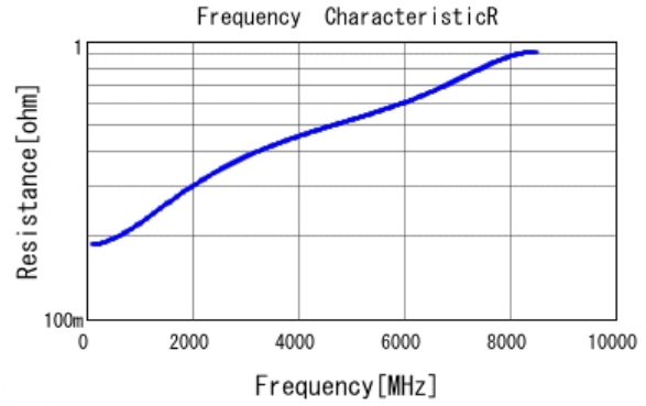
■ GRM0335C1E8R0CA01 R DCOV, 25degC
