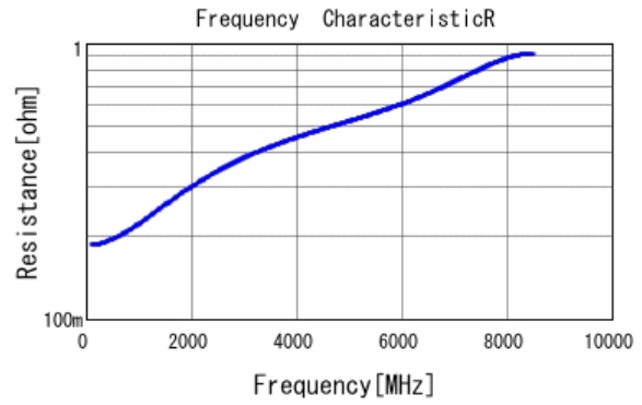
■ GRM0335C1E8R0DA01 R DCOV, 25degC
