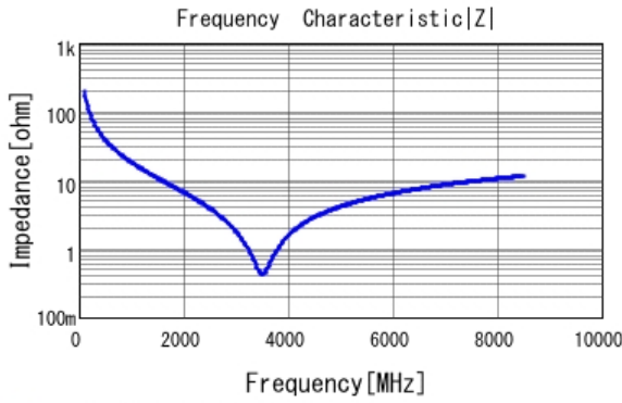
■ GRM0335C1E8R0DA01 |Z| DCOV, 25degC
