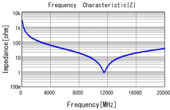
■ GRM0335C1ER60BA01 |Z| DCOV, 25degC
