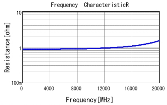
■ GRM0335C1ER60BA01 R DCOV, 25degC
