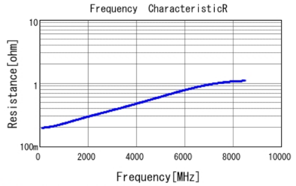
■ GRM0335C1H100GA01 R DCOV, 25degC
