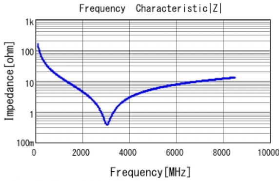
■ GRM0335C1H100GA01 |Z| DCOV, 25degC
