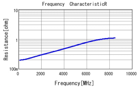
■ GRM0335C1H100JA01 R DCOV, 25degC
