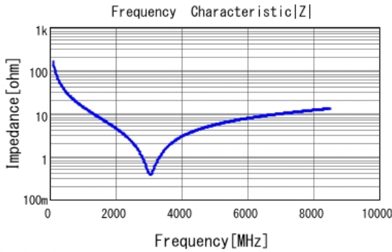
■ GRM0335C1H100JA01 |Z| DCOV, 25degC
