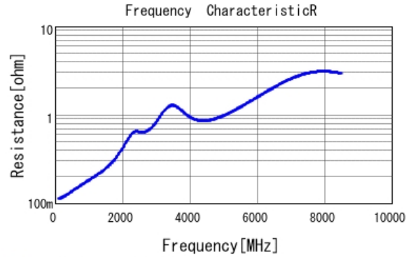
■ GRM0335C1H101GA01 R DCOV, 25degC
