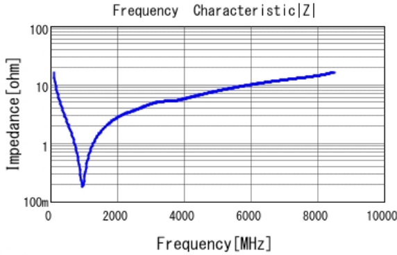
■ GRM0335C1H101GA01 |Z| DCOV, 25degC
