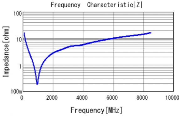
■ GRM0335C1H101JA01 |Z| DCOV, 25degC
