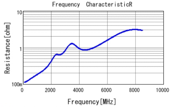
■ GRM0335C1H101JA01 R DCOV, 25degC
