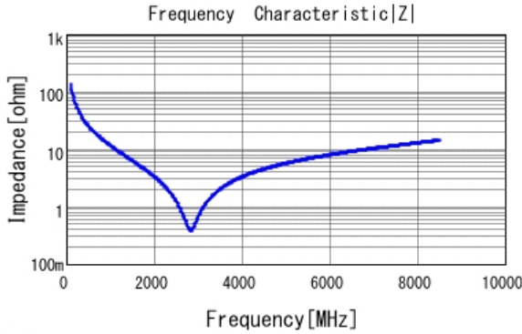
■ GRM0335C1H120JA01 |Z| DCOV, 25degC
