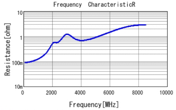
■ GRM0335C1H121GA01 R DCOV, 25degC
