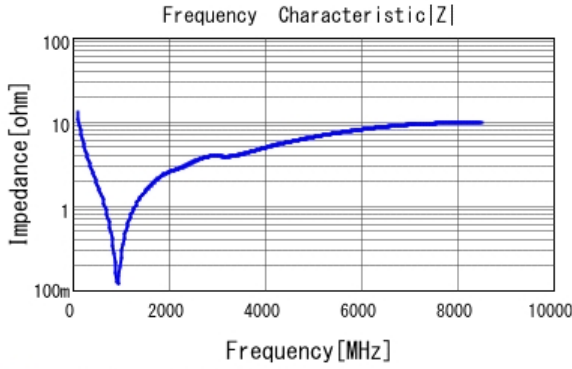
■ GRM0335C1H121GA01 |Z| DCOV, 25degC
