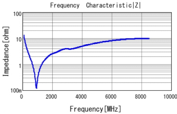
■ GRM0335C1H121JA01 |Z| DCOV, 25degC
