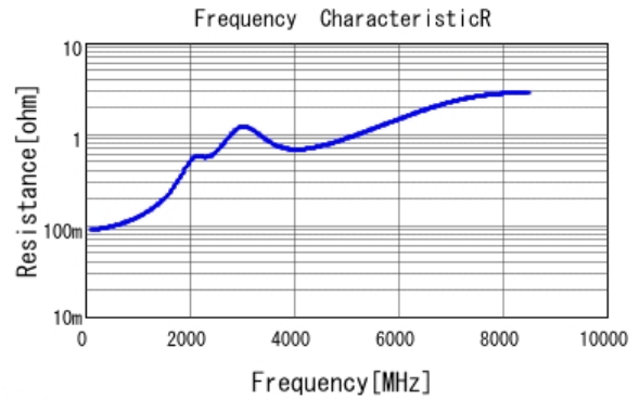
■ GRM0335C1H121JA01 R DCOV, 25degC
