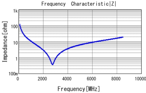
■ GRM0335C1H130JA01 |Z| DCOV, 25degC
