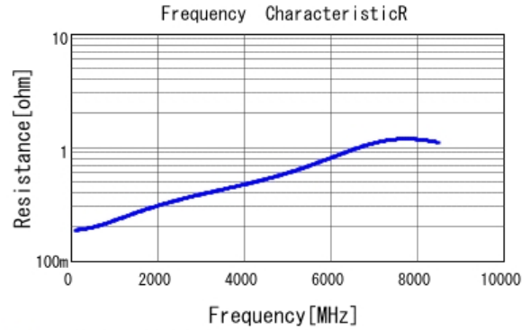
■ GRM0335C1H130JA01 R DCOV, 25degC
